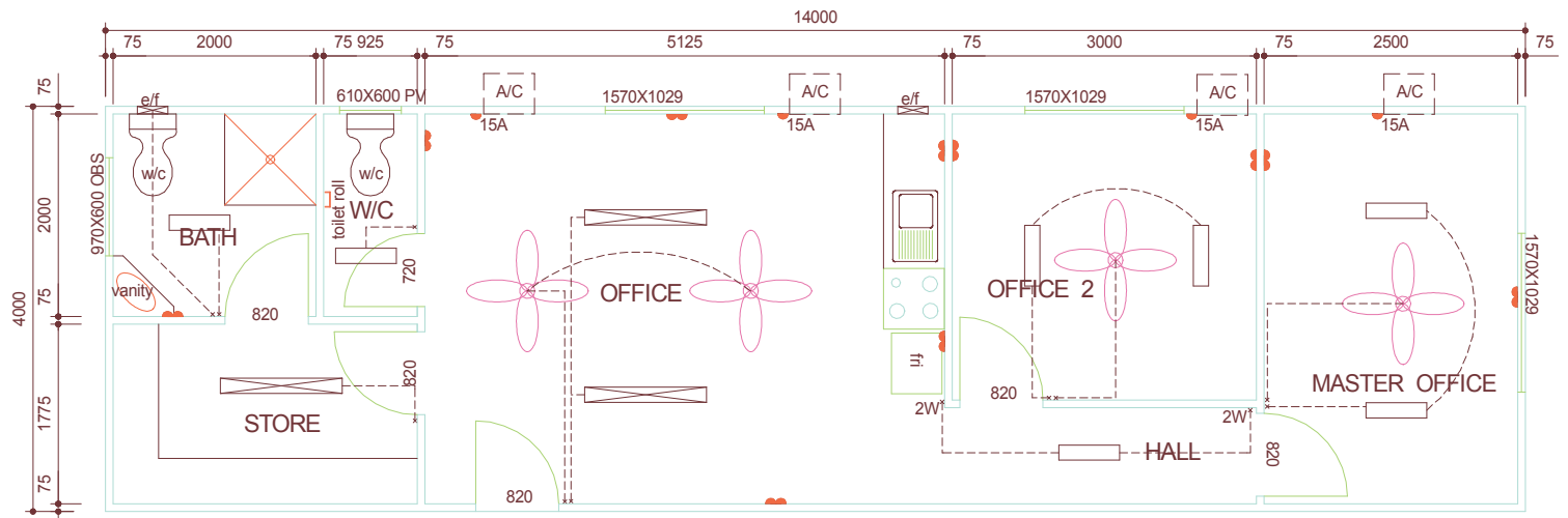
FLOOR PLAN
