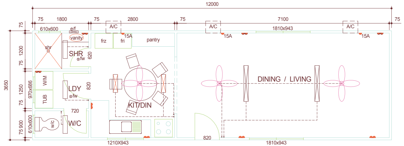
FLOOR PLAN
